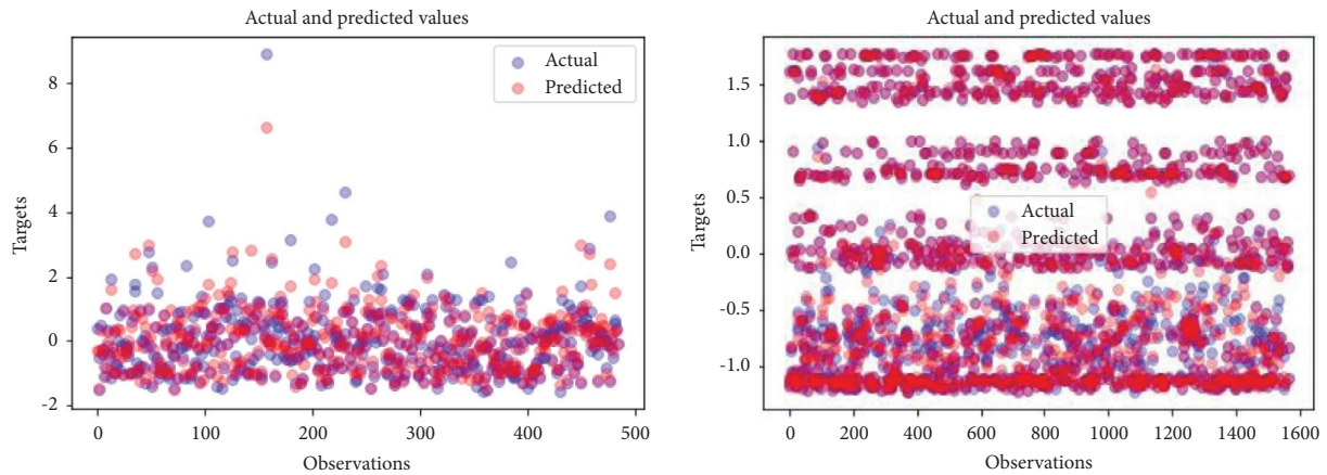
FIGURE 22: Scatter plots showing actual and predicted values for the imbalanced dataset (without using SMOTE) and balanced dataset (with using SMOTE) for Hyderabad-RFR.
